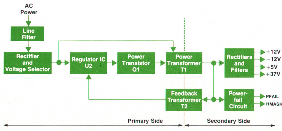
Fig. 1. Block diagram of the HP 2392A power supply.
