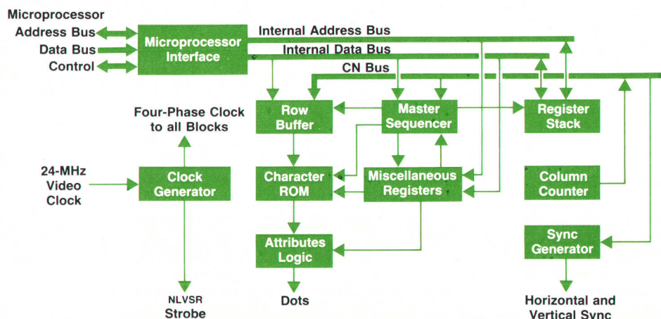
Fig. 4. Block diagram of the VLSI CRT controller chip used in the HP 2392A Terminal.
