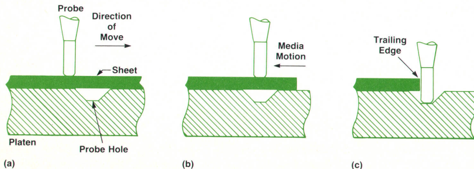
Fig. 3. Edge sensing. (a) A probe on the Z carriage bottoms on the media. (b) The Y carriage moves the probe over a hole in the platen. (c) As the trailing edge of the sheet passes, the probe drops into the hole.
