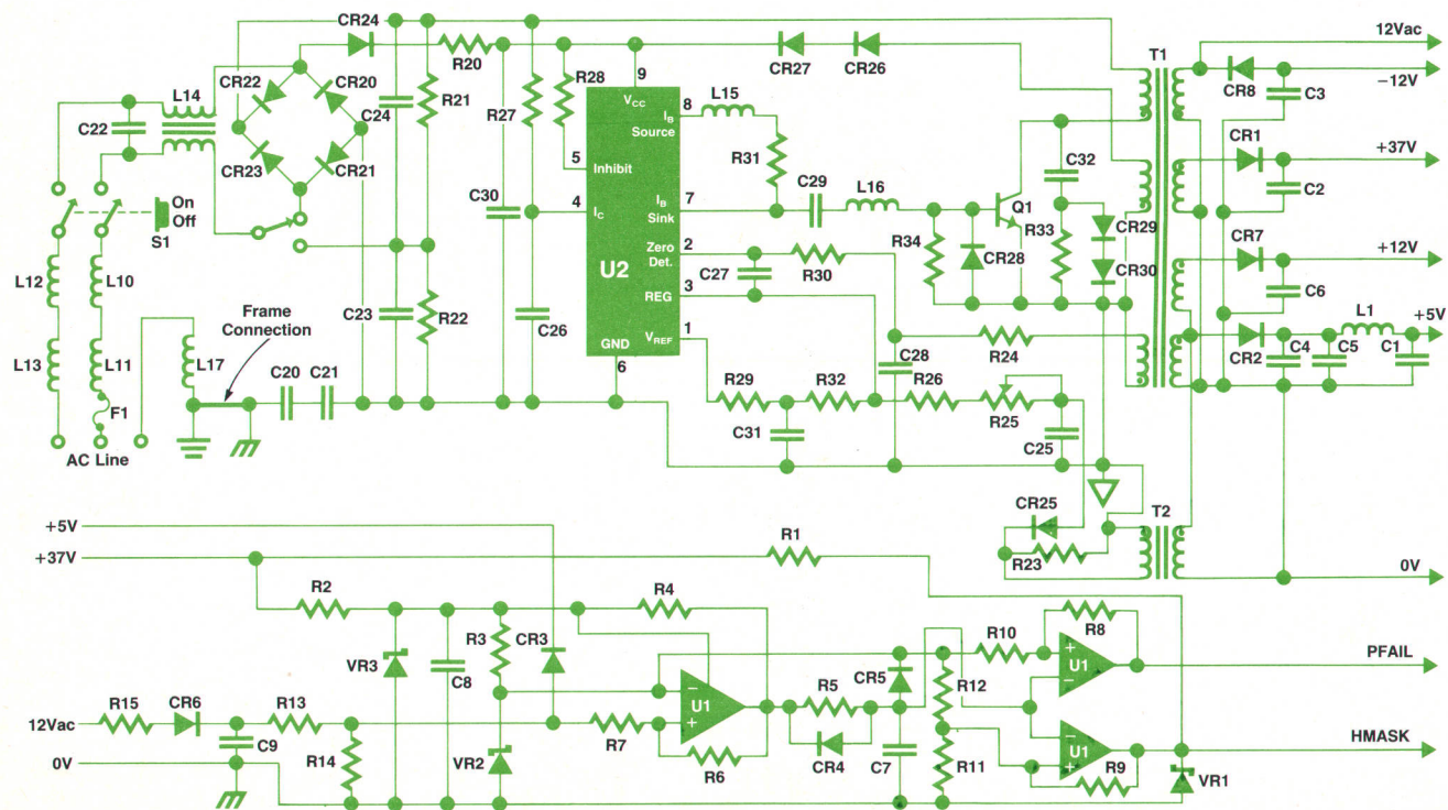
Fig. 2. HP 2392A power supply schematic diagram.
