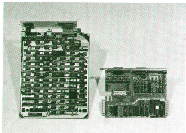
Fig. 2. The HP 2392A's logic board (right) has only one fourth as many chips as earlier HP designs (left).
