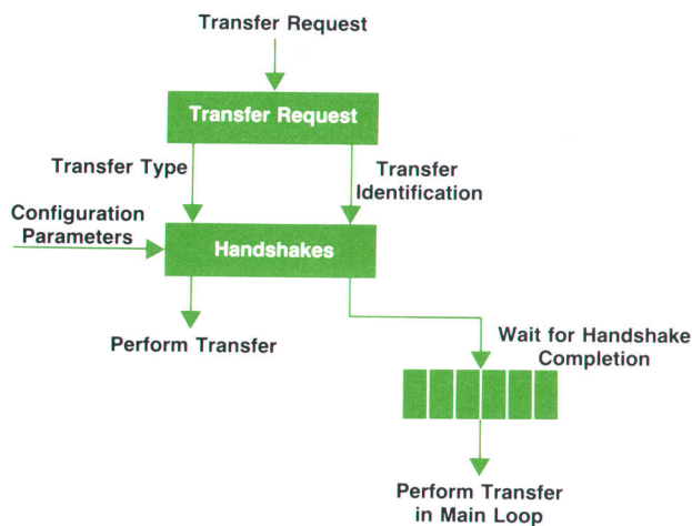
Fig. 4. Block mode transfer handling in the HP 2392A.
